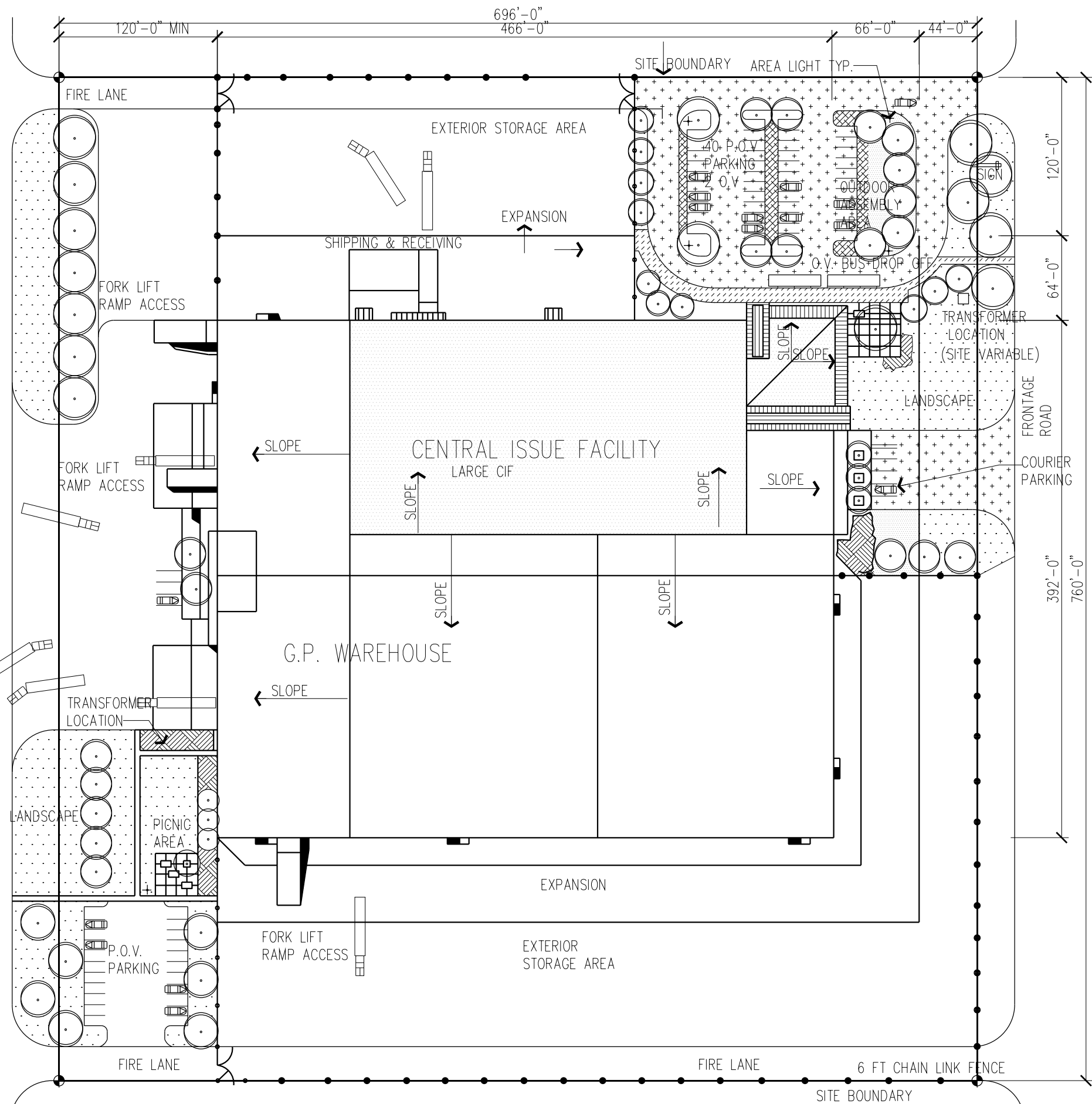
1 CENTRAL ISSUE FACILITY SITE LAYOUT (LARGE) SCALE: N.T.S.
